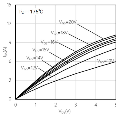
Fig5. Typical output characteristic
