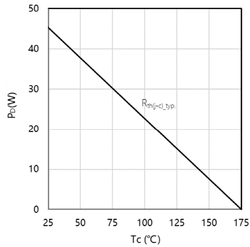
Fig2. Power dissipation
