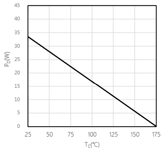
Fig2. Power dissipation
