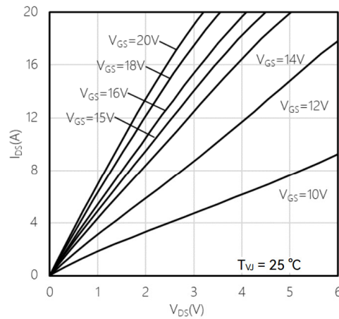
Fig4. Typical output characteristic
