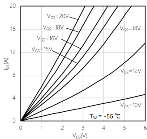
Fig3. Typical output characteristic
