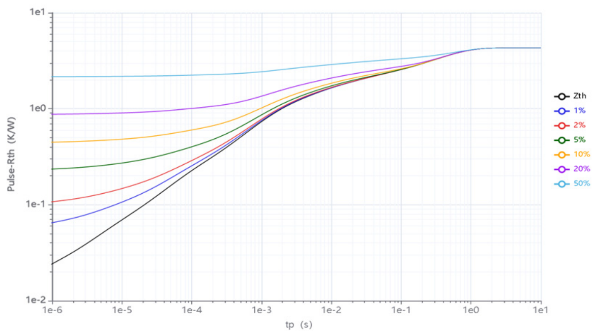
Fig24. Transient thermal resistance (MOSFET)
