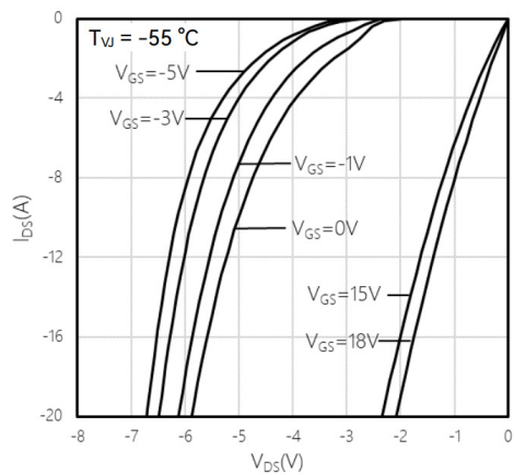
Fig11. Typical reverse drain current as function of reverse drain voltage
