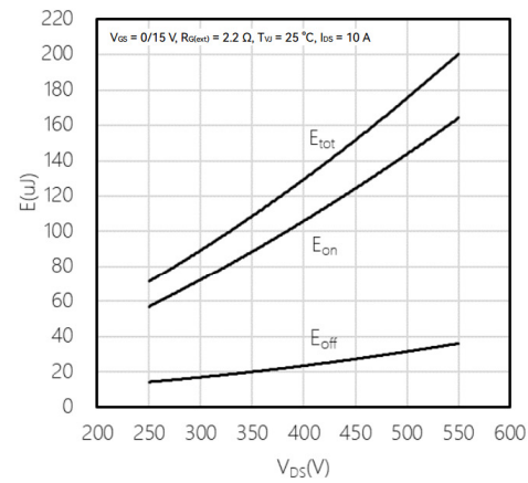
Fig20. Typical switching energy losses as a function of V_{DS} , 2nd device own body diode: V_{GS} = -5\text{ V}
