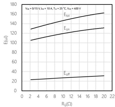
Fig16. Typical switching energy losses as a function of gate resistance, 2nd device own body diode: VGS = -5V
