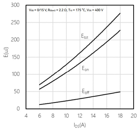
Fig19. Typical switching energy losses as a function of I_{DS} , 2nd device own body diode: V_{GS} = -5\text{ V}
