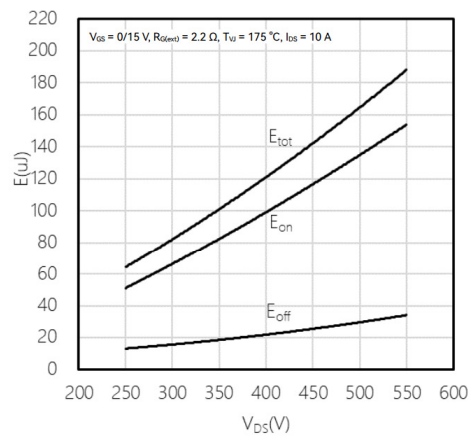
Fig21. Typical switching energy losses as a function of V_{DS} , 2nd device own body diode: V_{GS} = -5\text{ V}
