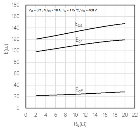
Fig17. Typical switching energy losses as a function of gate resistance, 2nd device own body diode: VGS = -5V
