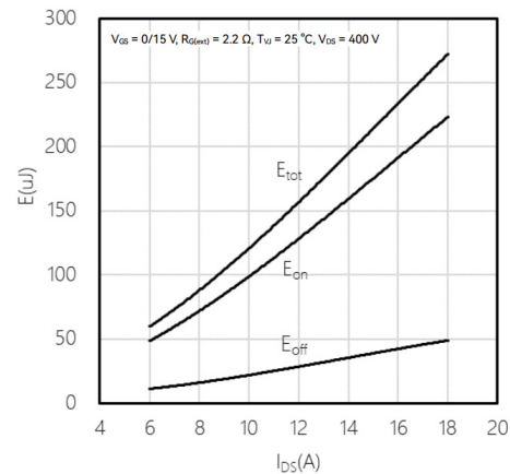
Fig18. Typical switching energy losses as a function of IDS, 2nd device own body diode: VGS = -5V
