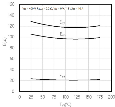
Fig15. Typical switching energy as a function of junction temperature, 2nd device own body diode: VGS = -5V
