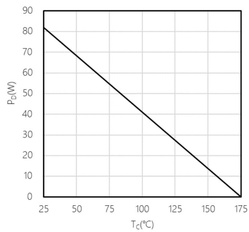
Fig2. Power dissipation
