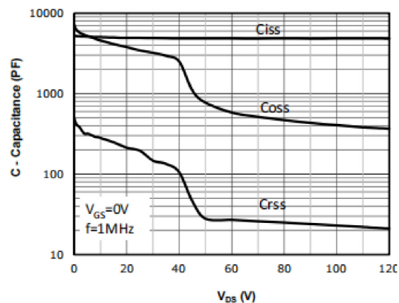
Fig 6: Capacitance Characteristics
