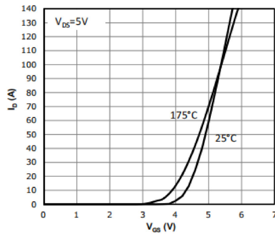
Fig 2 : Transfer Characteristics
