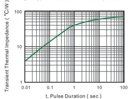
Fig.5- Typical Transient Thermal Impedance
