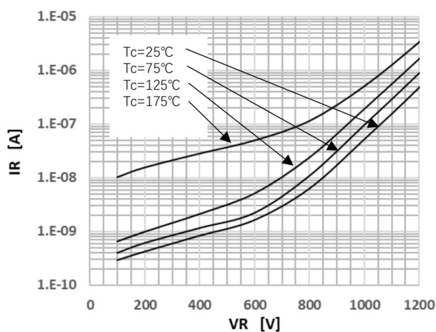
Figure 2 Reverse Characteristics
