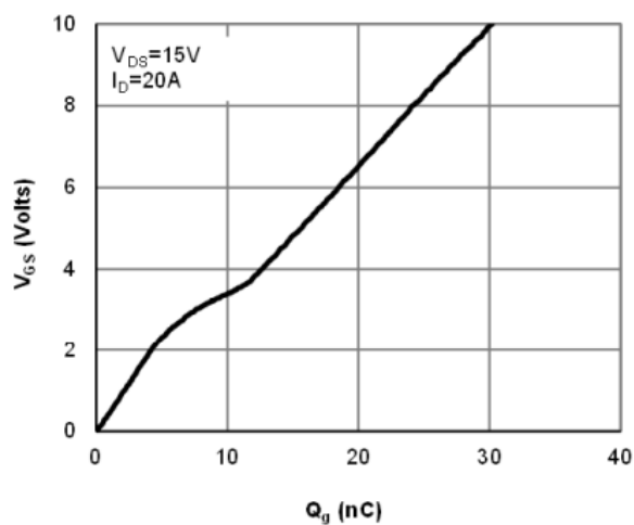
Figure 7: Gate-Charge Characteristics
