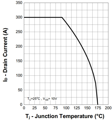
2. Current Capability
