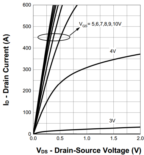
5. Output Characteristics
