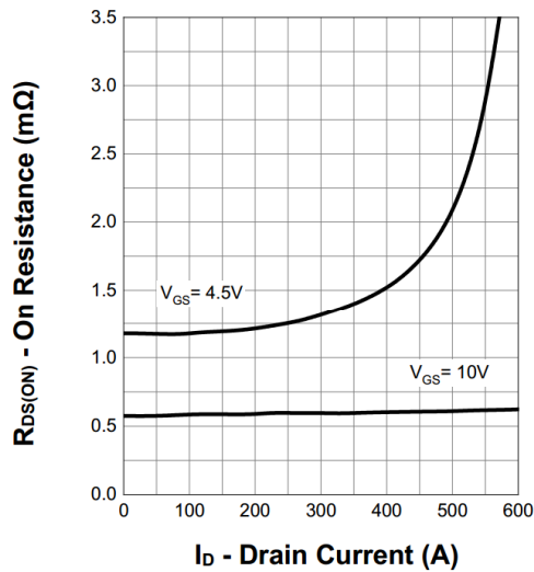
6. On Resistance
