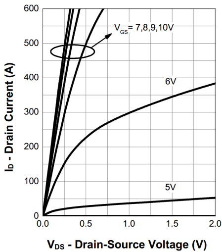
5. Output Characteristics
