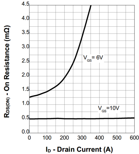
6. On Resistance
