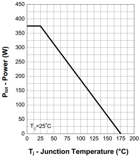
1. Power Capability
