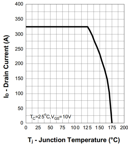
2. Current Capability
